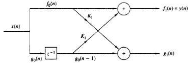
Figure 3: Single Stage Lattice Fiter.
