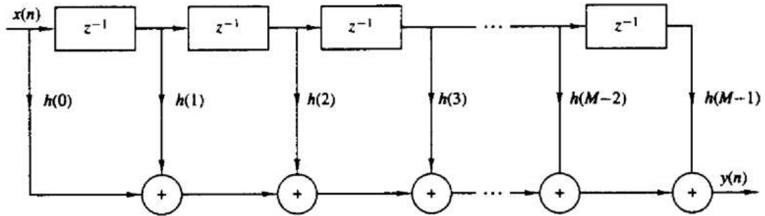
Figure 1: Direct Form Structure of FIR system.
